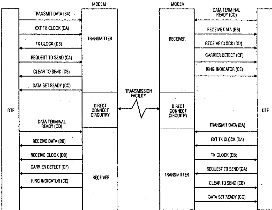
Figure 2-2 Digital Interface Signals
